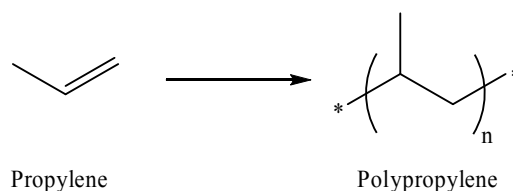
Figure 1: Propylene polymerisation
